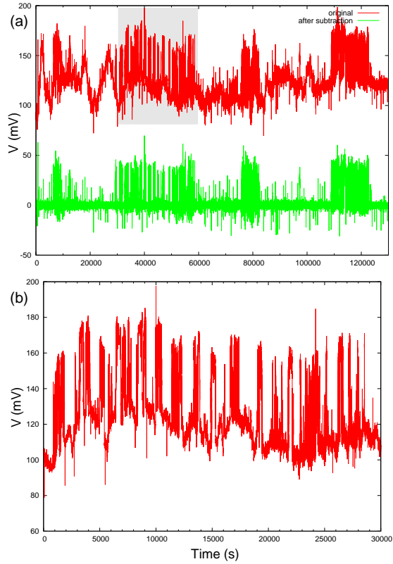
FIG. 2: (color online) (a) The red color represents the original record of the SES activity at a station close to Pirgos town in Western Greece, which lasted from 29 February to 2 March 2008. This SES activity was superimposed on a pseudosinusoidal background, due to MT variations, which are evident in the left part of the figure. After subtracting the MT background -by means of the procedure described in Ref. 42- the green signal of dichotomous nature remains which constitutes the true precursory signal, i.e., the SES activity. (b) An almost 8.3 h excerpt of the original record (shaded in (a)) is plotted here in expanded time scale.
