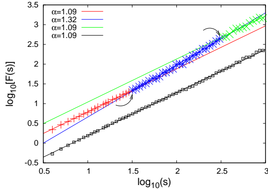
FIG. 3: (color online) The DFA plot resulting from the analysis of an excerpt -shaded in Fig. 2(a)- of the original time series of the SES activity plotted in red in Fig. 2(a) superimposed on MT variations. It comprises three parts -shown in red, blue and green- two of which, i.e., the ones corresponding to the shortest and the largest scales, are depicted in red and green, respectively. The two cross-overs observed are marked with arrows. For the sake of comparison, the plot in black depicts the results deduced from the DFA analysis (shifted vertically for the sake of clarity) when considering the SES activity alone, i.e., the signal of dichotomous nature plotted in green in Fig. 2(a)
