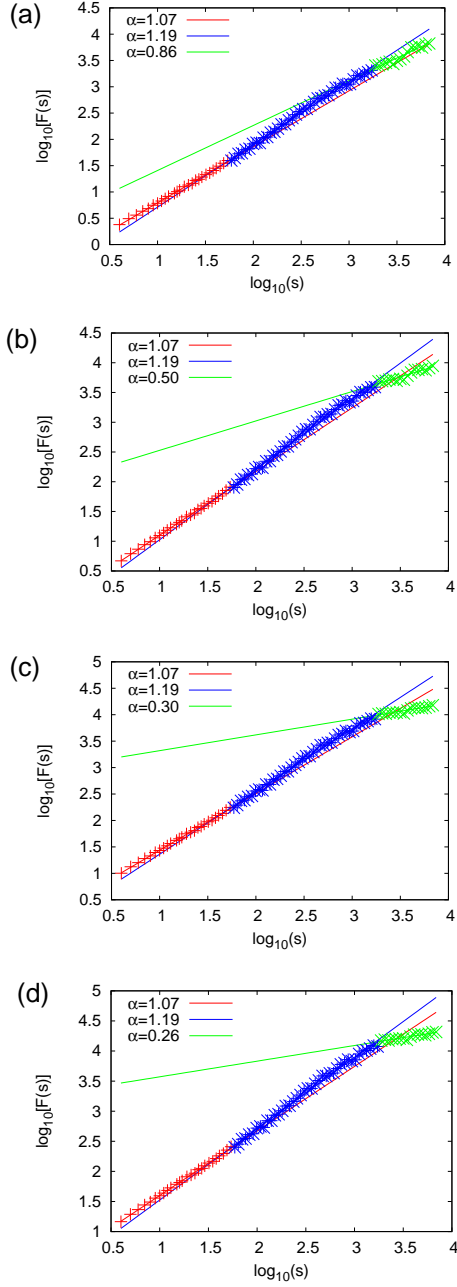
FIG. 4: (color online) The DFA plots resulting from the analyses of excerpts of SES activities that precede EQs of various magnitudes M_w=6.5 (a), 7.5 (b), 8.5 (c) and 9.0 (d) (see the text)
